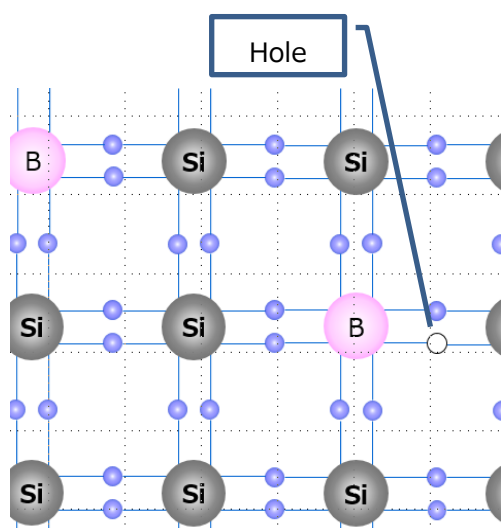
Figure 3.2 p-type semiconductor
