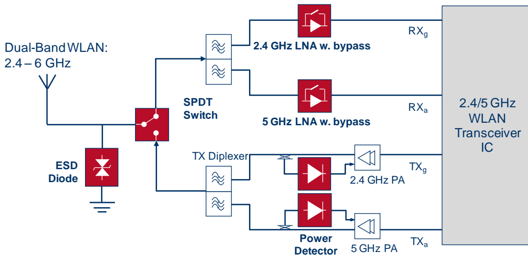
WLAN Application Example 2: Dual-band (2.4–6.0 GHz) WLAN (IEEE 802.11a/b/g/n/ac) FE
