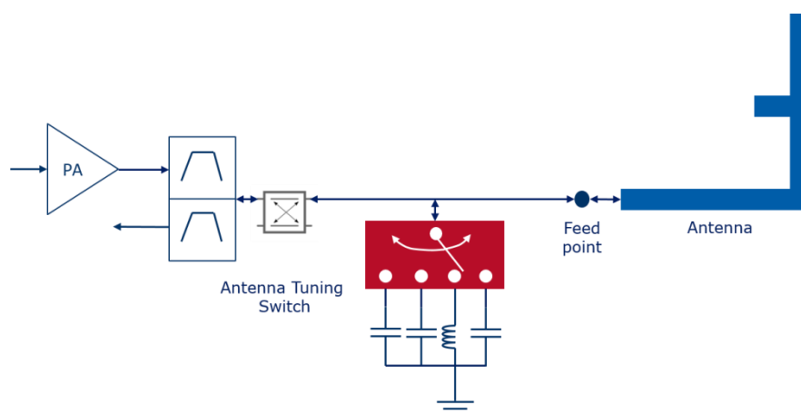
Antenna impedance matching
