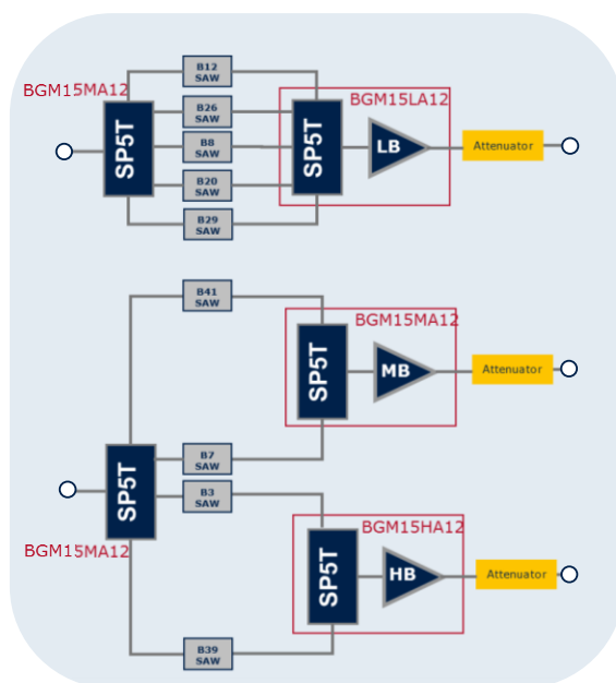
Block diagram and implemented hardware for verification
