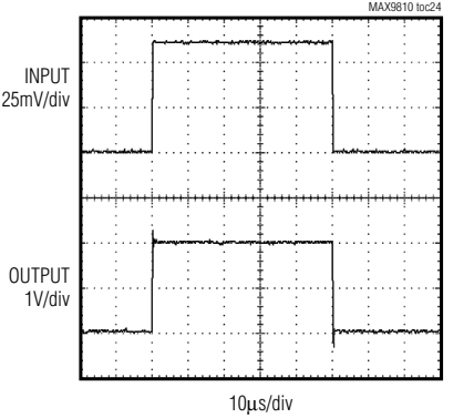
DRIVING MAXIMUM CAPACITIVE LOAD WAVEFORM
