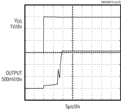
POWER-UP WAVEFORM
